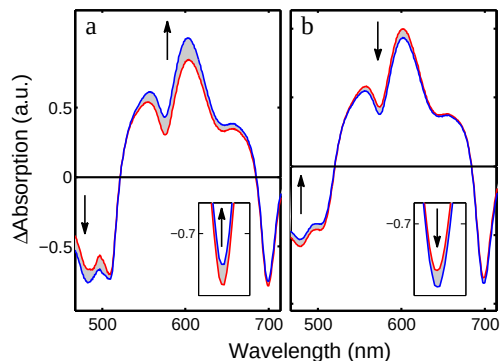
Figure 7.5: The transient spectra at 8 ps probe delay using TL pulse (red line) and the found optimal shapes (blue line). Panel a: IC/ET optimisation. Population transfer increases, IC increases and the ET reduces slightly. Panel b: ET/IC optimisation. Population transfer decreases, IC decreases and the ET increases. Insets: Zoom-in to ET signals at \sim 700 nm. The arrows indicate the change from the TL to the optimal pulse shapes.
