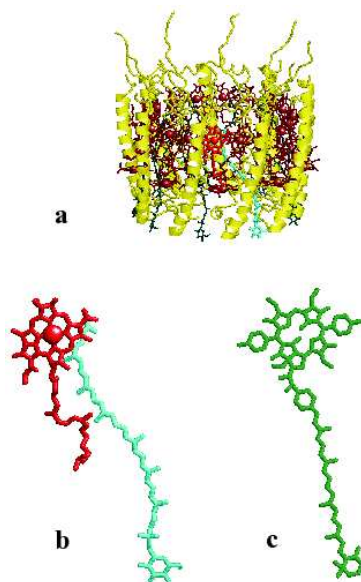
Figure 6.1: Structure of LH2 pigments as compared to the dyad. Panel a: LH2. Panel b: expansion of two highlighted pigments in Panel a (the carotenoid donor in blue and the porphyrin acceptor in red). Panel c: schematic structure of the carotenoporphyrin dyad; the donor and acceptor are chemically bridged by an amide link.
